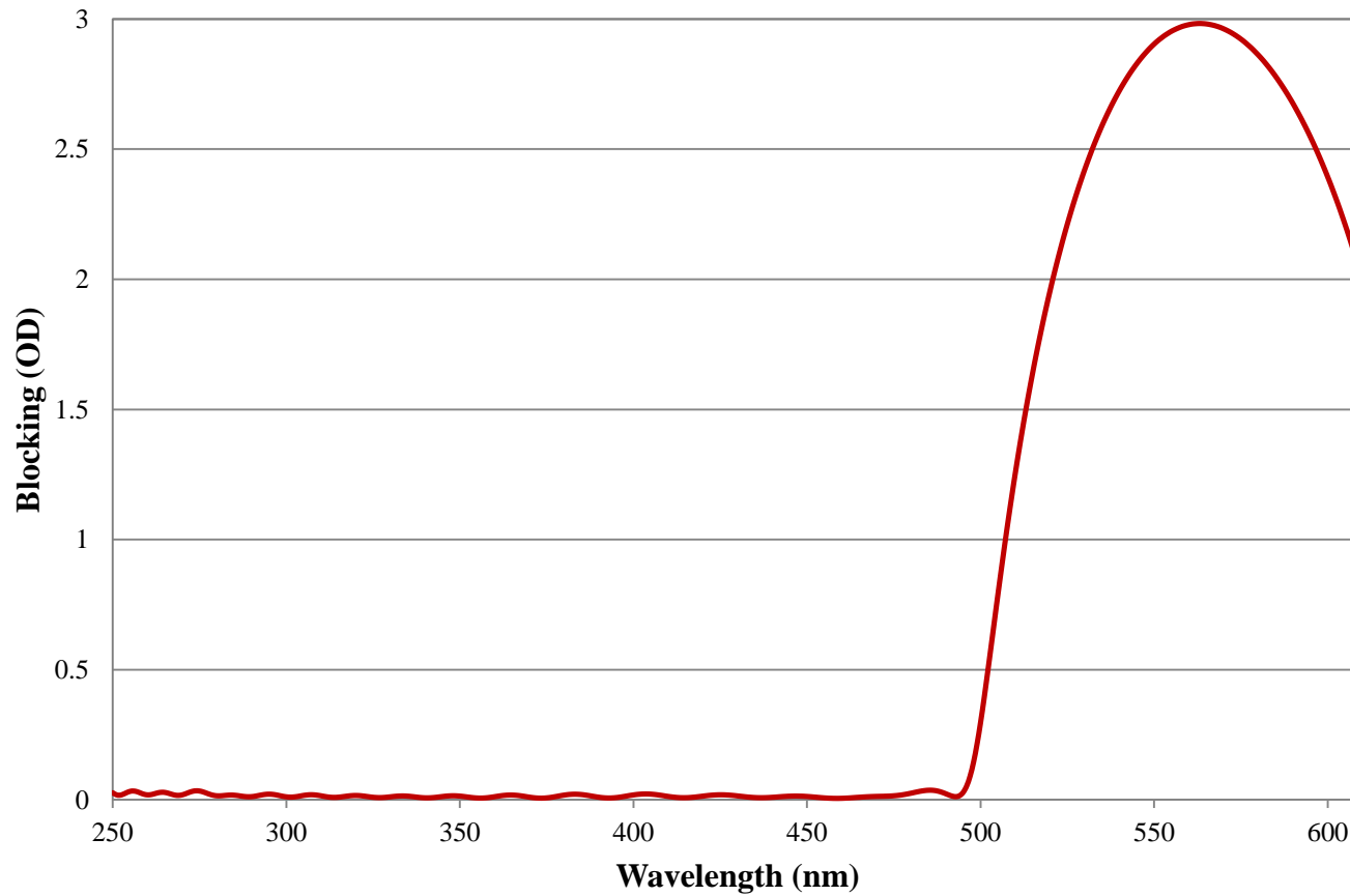
500nm Techspec Shortpass Filter: OD >2.0 Coating Performance FOR REFERENCE ONLY
