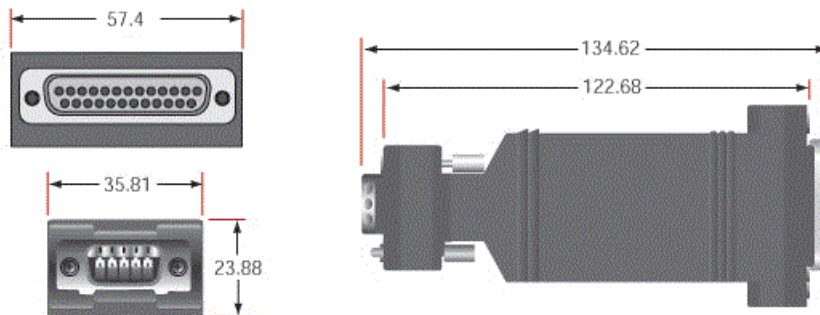
D-to-A Converter #55-232
