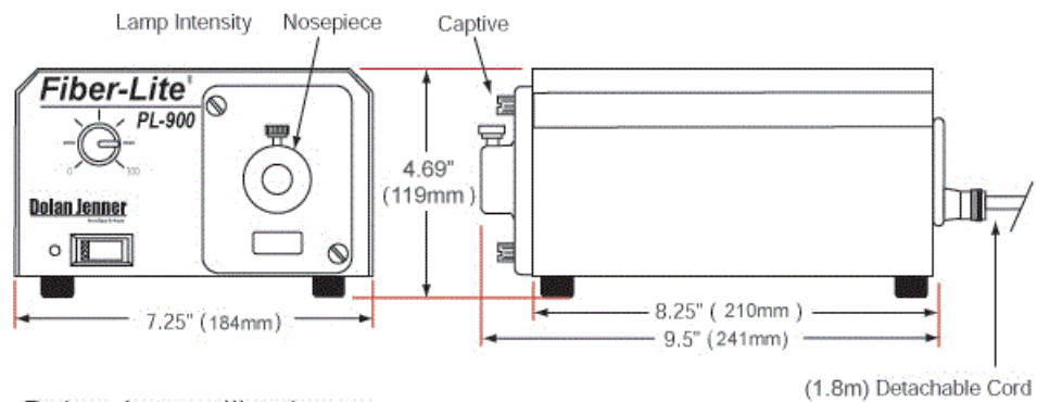
Dolan-Jenner Illuminator
