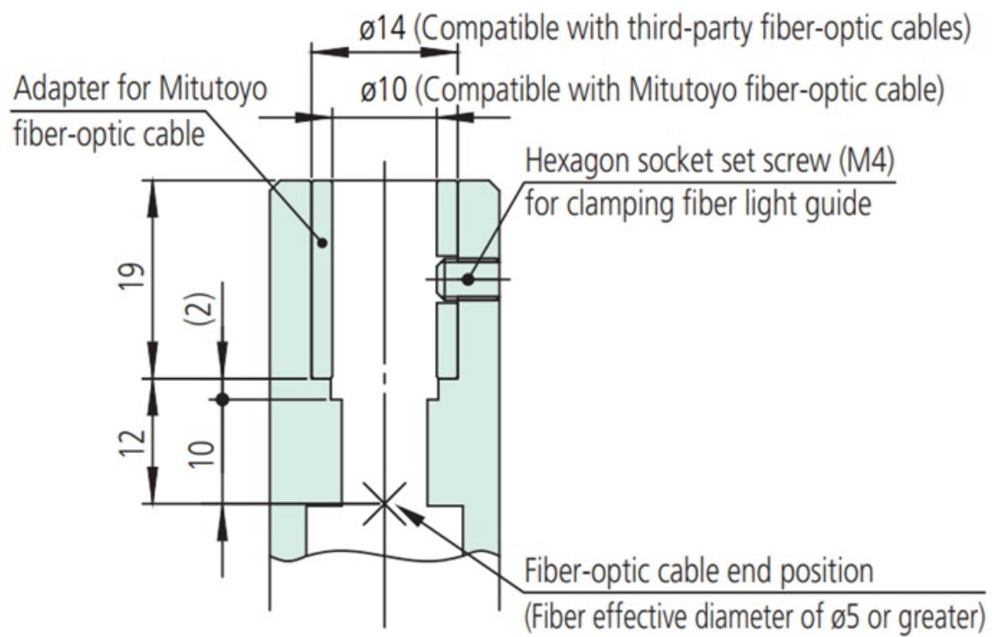
Detail of fiber mount
