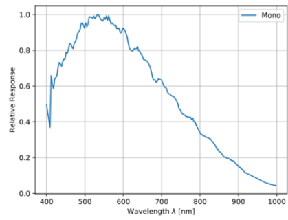
GMAX2518 Sensor QE Curve
