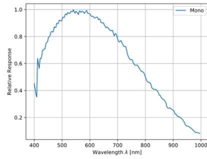
IMX547 Sensor QE Curve
