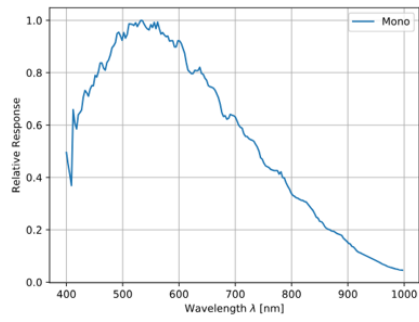
GMAX2509 Sensor QE Curve
