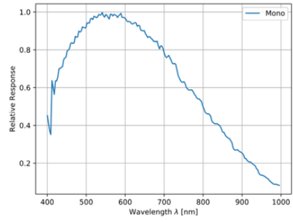
IMX545 Sensor QE Curve
