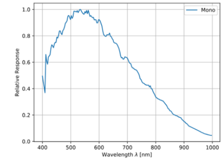
GMAX2505 Sensor QE Curve
