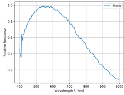
IMX546 Sensor QE Curve
