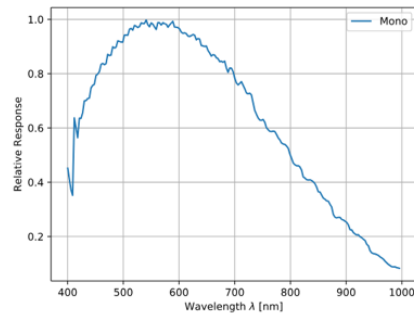
E2525A Sensor QE Curve
