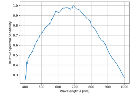
IMX900 Sensor QE Curve
