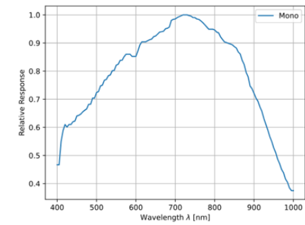
IMX676 Sensor QE Curve
