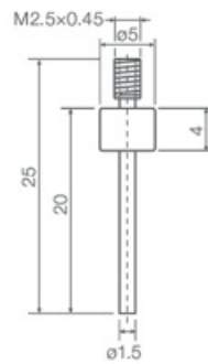
Pin attachment
