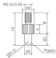
Roller attachment
