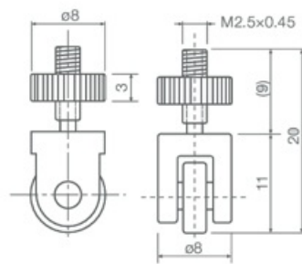
Roller attachment
