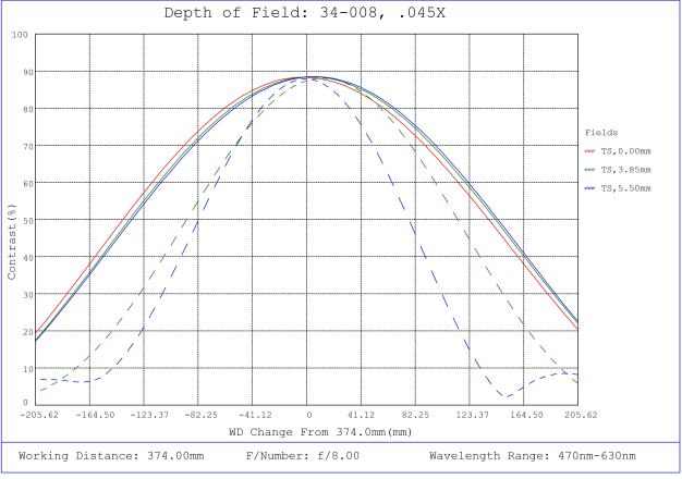
#34-008, 0.045X, 2/3" C-Mount TitanTL® Telecentric Lens, Depth of Field Plot, 374mm Working Distance, f8
