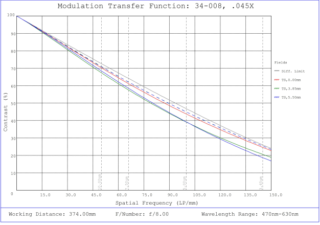
#34-008, 0.045X, 2/3" C-Mount TitanTL® Telecentric Lens, Modulated Transfer Function (MTF) Plot, 374mm Working Distance, f8
