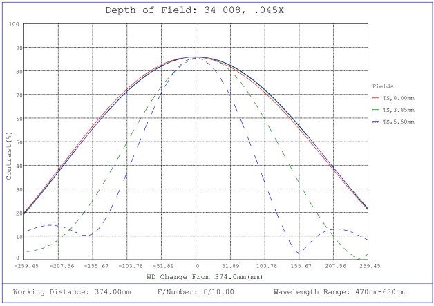
#34-008, 0.045X, 2/3" C-Mount TitanTL® Telecentric Lens, Depth of Field Plot, 374mm Working Distance, f10
