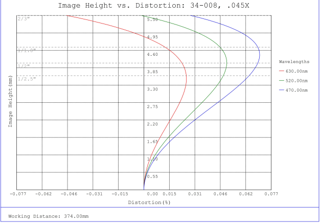
#34-008, 0.045X, 2/3" C-Mount TitanTL® Telecentric Lens, Distortion Plot
