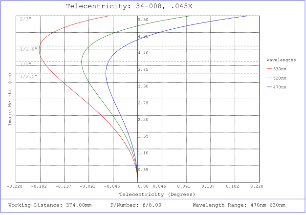
#34-008, 0.045X, 2/3" C-Mount TitanTL® Telecentric Lens, Telecentricity Plot
