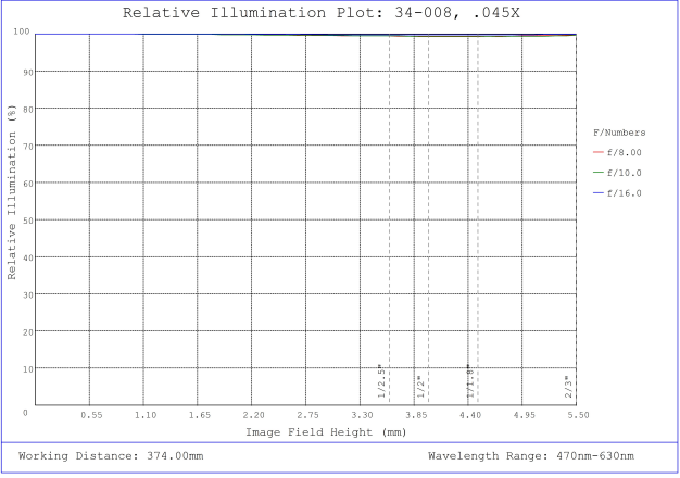
#34-008, 0.045X, 2/3" C-Mount TitanTL® Telecentric Lens, Relative Illumination Plot
