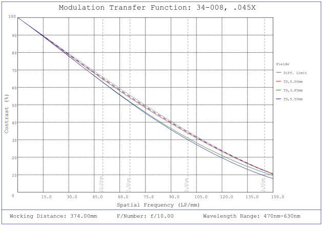
#34-008, 0.045X, 2/3" C-Mount TitanTL® Telecentric Lens, Modulated Transfer Function (MTF) Plot, 374mm Working Distance, f10
