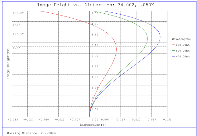
#34-002, 0.050X, 1/1.8" C-Mount TitanTL® Telecentric Lens, Distortion Plot
