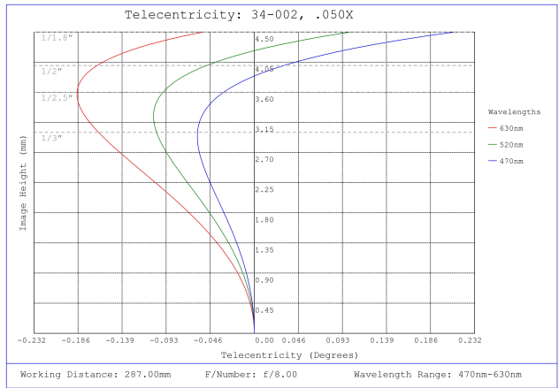
#34-002, 0.050X, 1/1.8" C-Mount TitanTL® Telecentric Lens, Telecentricity Plot
