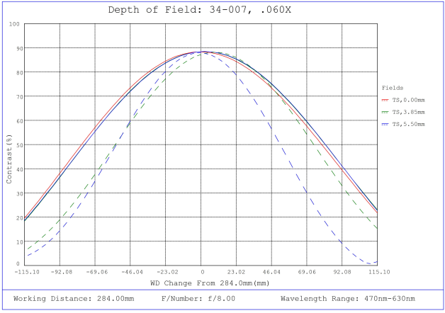
#34-007, 0.060X, 2/3" C-Mount TitanTL® Telecentric Lens, Depth of Field Plot, 284mm Working Distance, f8
