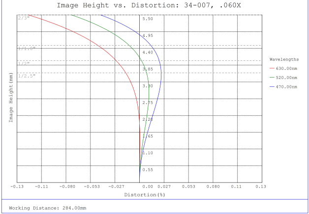
#34-007, 0.060X, 2/3" C-Mount TitanTL® Telecentric Lens, Distortion Plot
