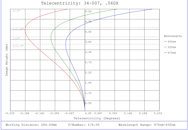
#34-007, 0.060X, 2/3" C-Mount TitanTL® Telecentric Lens, Telecentricity Plot
