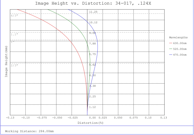
#34-017, 0.124X, 4/3" C-Mount TitanTL® Telecentric Lens, Distortion Plot
