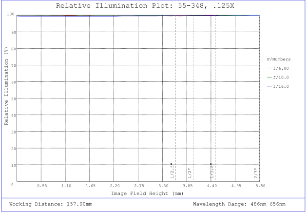
#55-348, 0.125X, 2/3" GoldTL™ Telecentric Lens, Relative Illumination Plot
