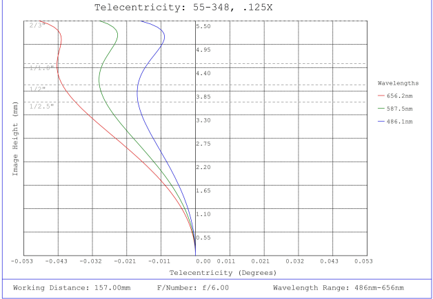
#55-348, 0.125X, 2/3" GoldTL™ Telecentric Lens, Telecentricity Plot
