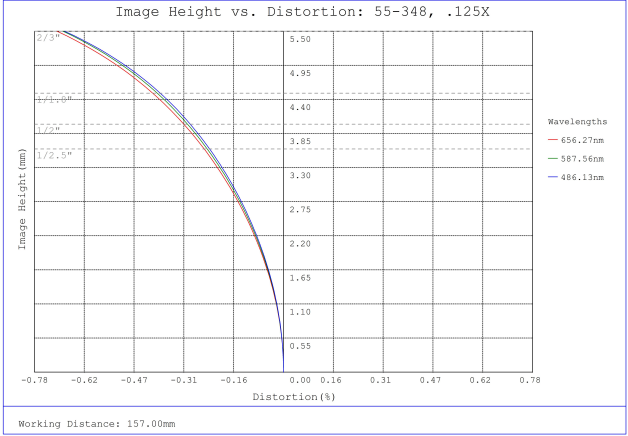
#55-348, 0.125X, 2/3" GoldTL™ Telecentric Lens, Distortion Plot
