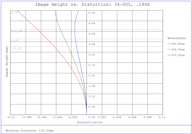
#34-005, 0.184X, 2/3" C-Mount TitanTL® Telecentric Lens, Distortion Plot
