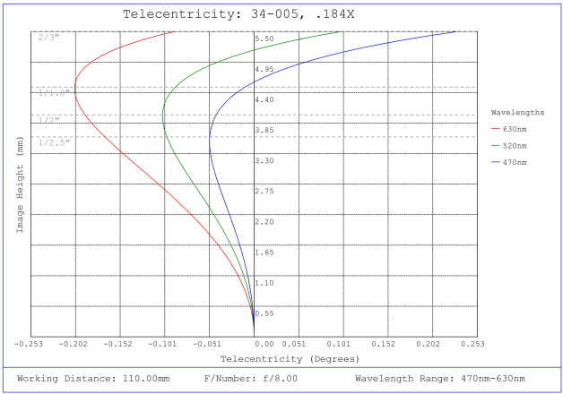
#34-005, 0.184X, 2/3" C-Mount TitanTL® Telecentric Lens, Telecentricity Plot
