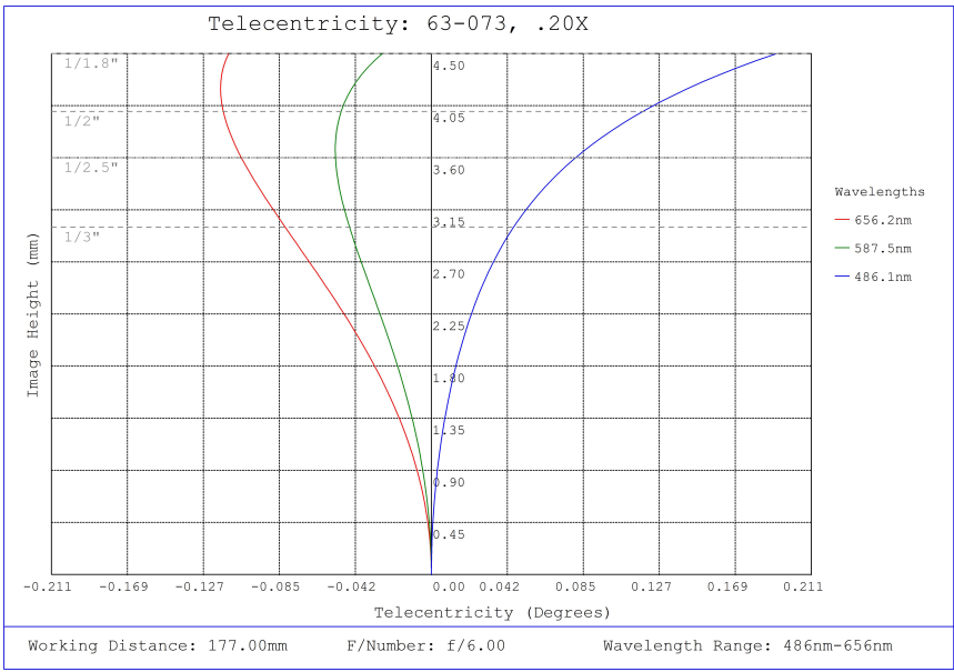
#63-073, 0.20X SilverTL™ Telecentric Lens, Telecentricity Plot
