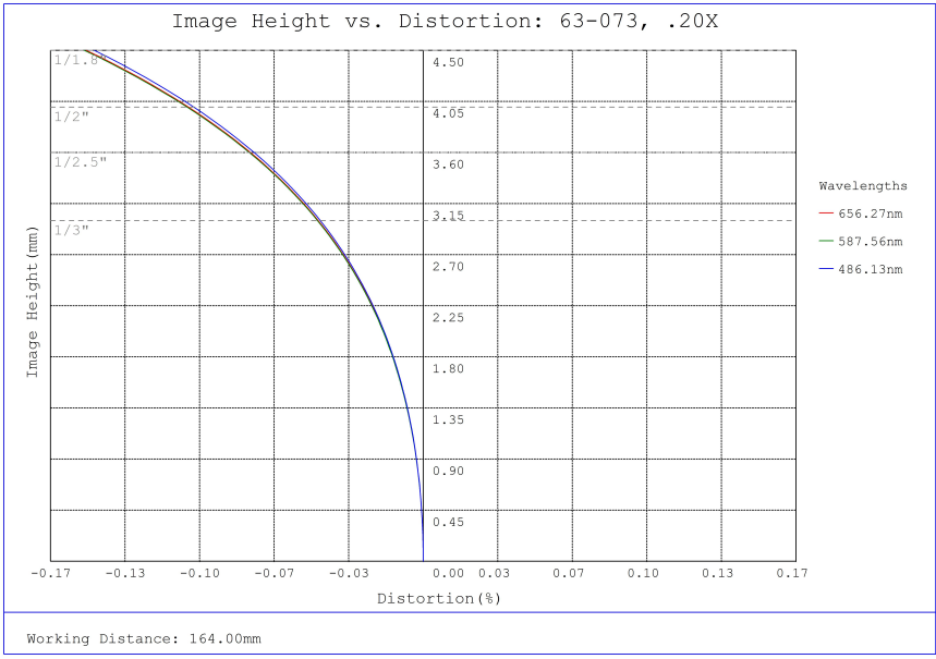
#63-073, 0.20X SilverTL™ Telecentric Lens, Distortion Plot
