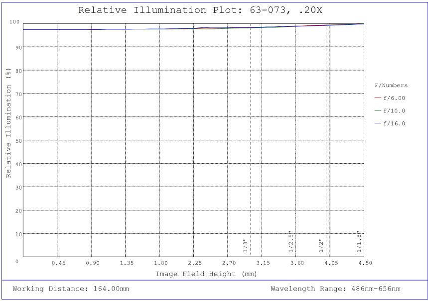
#63-073, 0.20X SilverTL™ Telecentric Lens, Relative Illumination Plot
