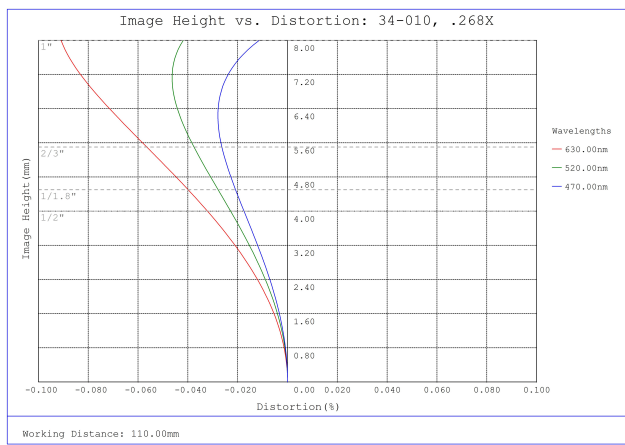
#34-010, 0.268X, 1" C-Mount TitanTL® Telecentric Lens, Distortion Plot
