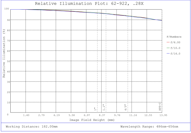
#62-922, 0.28X, 28.7mm F-Mount PlatinumTL™ Telecentric Lens, Relative Illumination Plot
