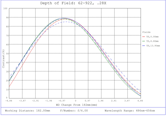
#62-922, 0.28X, 28.7mm F-Mount PlatinumTL™ Telecentric Lens, Depth of Field Plot, 182mm Working Distance, f6
