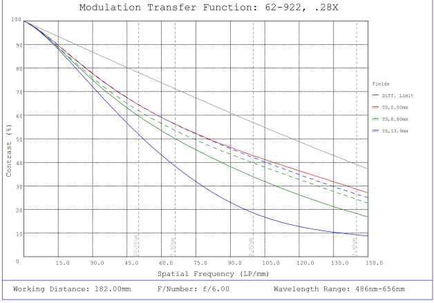
#62-922, 0.28X, 28.7mm F-Mount PlatinumTL™ Telecentric Lens, Modulated Transfer Function (MTF) Plot, 182mm Working Distance, f6
