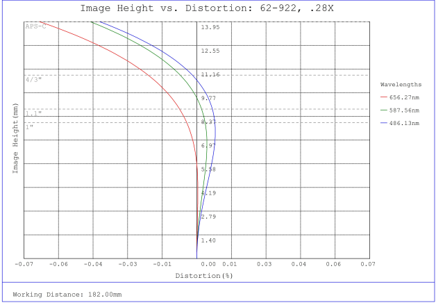
#62-922, 0.28X, 28.7mm F-Mount PlatinumTL™ Telecentric Lens, Distortion Plot
