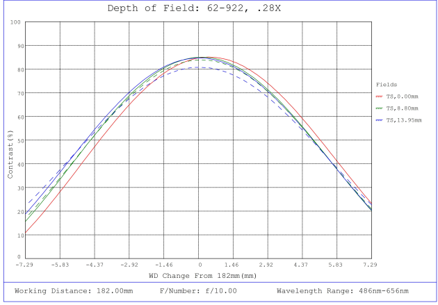
#62-922, 0.28X, 28.7mm F-Mount PlatinumTL™ Telecentric Lens, Depth of Field Plot, 182mm Working Distance, f10
