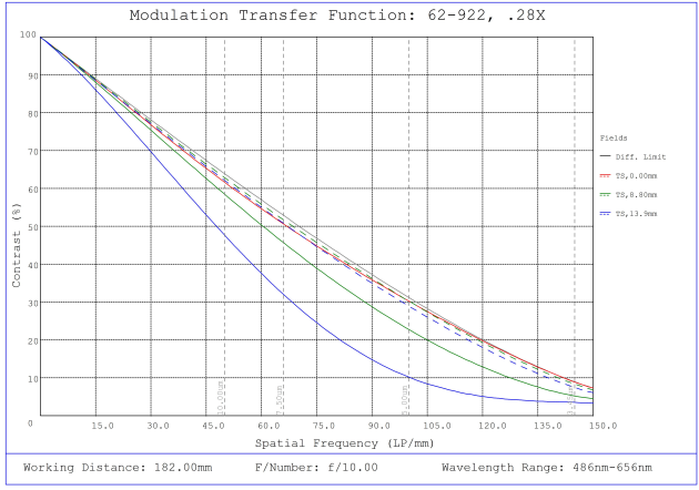
#62-922, 0.28X, 28.7mm F-Mount PlatinumTL™ Telecentric Lens, Modulated Transfer Function (MTF) Plot, 182mm Working Distance, f10
