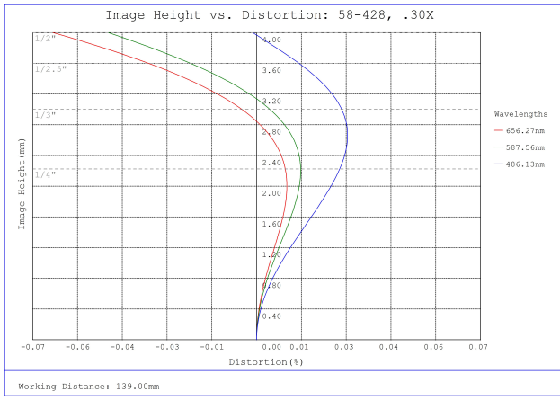
#58-428, 0.30X SilverTL™ Telecentric Lens, Distortion Plot
