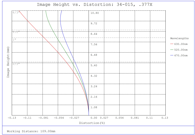
#34-015, 0.377X, 4/3" C-Mount TitanTL® Telecentric Lens, Distortion Plot
