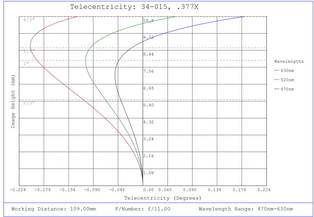
#34-015, 0.377X, 4/3" C-Mount TitanTL® Telecentric Lens, Telecentricity Plot
