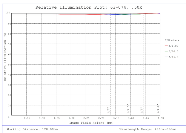
#63-074, 0.50X SilverTL™ Telecentric Lens, Relative Illumination Plot
