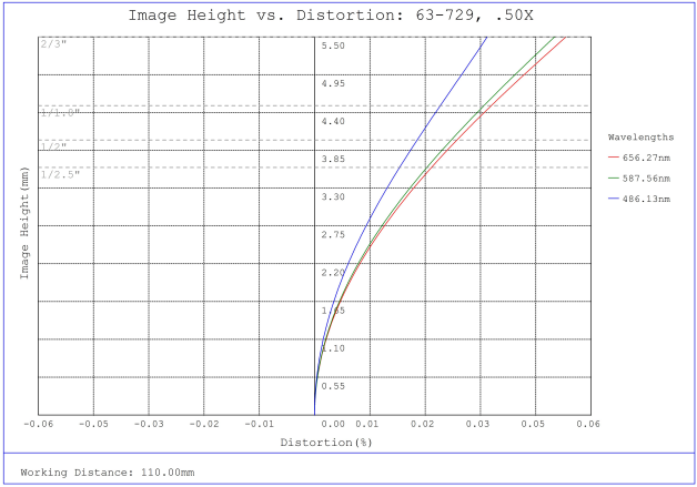
#63-729, 0.5X, 110mm WD CompactTL™ Telecentric Lens, Distortion Plot
