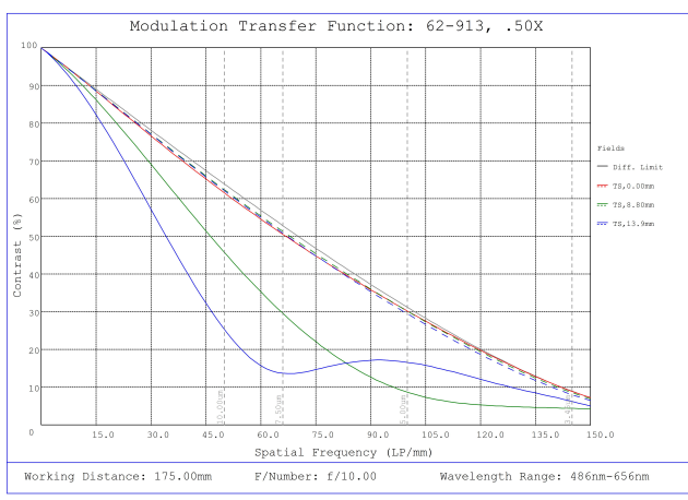
#62-913, 0.5X, 28.7mm M42 x 1.0 (6.56mm) PlatinumTL™ Telecentric Lens, Modulated Transfer Function (MTF) Plot, 175mm Working Distance, f10
