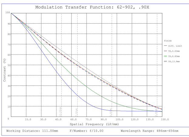
#62-902, 0.9X, 28.7mm F-Mount PlatinumTL™ Telecentric Lens, Modulated Transfer Function (MTF) Plot, 111mm Working Distance, f10
