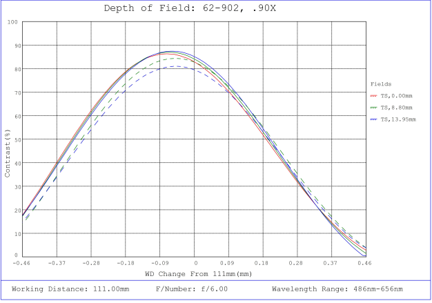
#62-902, 0.9X, 28.7mm F-Mount PlatinumTL™ Telecentric Lens, Depth of Field Plot, 111mm Working Distance, f6
