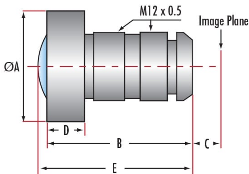
Infinite Conjugate M12 Imaging Lenses
