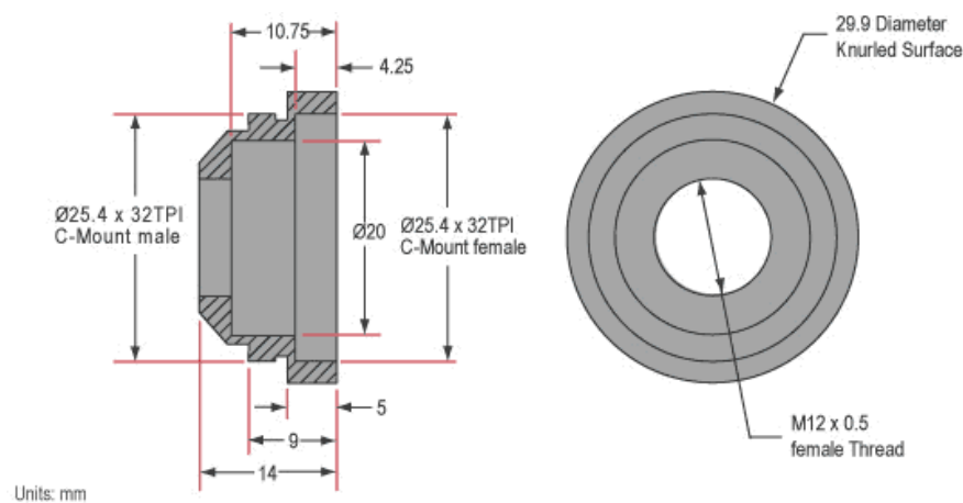
C-Mount Adapter (#53-675)
