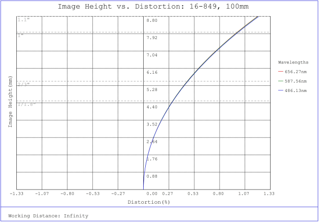
#16-849, 100mm, f/4 Athermal Lens, Distortion Plot
