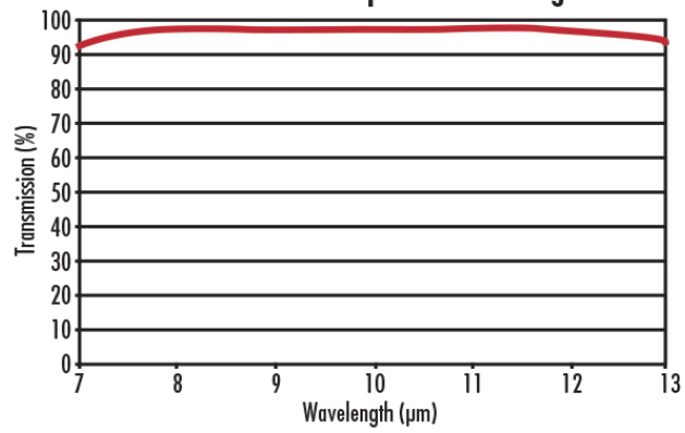
Silicon with 8-12 \mu m BBAR Coating
