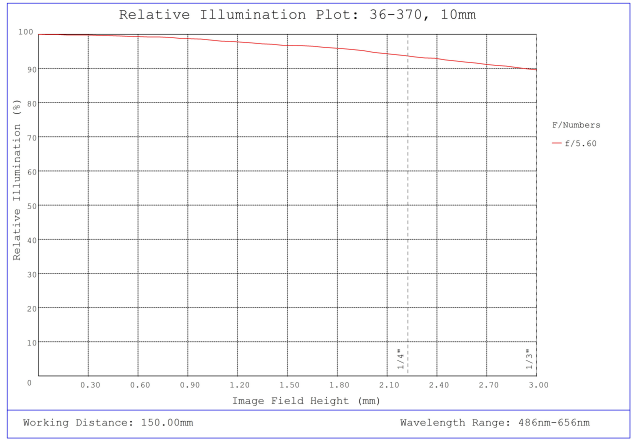
#36-370, 10mm FL f/5.6, Rugged Blue Series M12 Lens, Relative Illumination Plot
