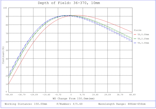
#36-370, 10mm FL f/5.6, Rugged Blue Series M12 Lens, Depth of Field Plot, 150mm Working Distance, f5.6
