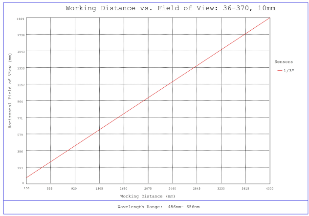
#36-370, 10mm FL f/5.6, Rugged Blue Series M12 Lens, Working Distance versus Field of View Plot
