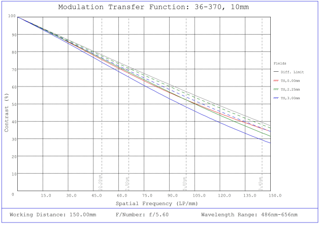
#36-370, 10mm FL f/5.6, Rugged Blue Series M12 Lens, Modulated Transfer Function (MTF) Plot, 150mm Working Distance, f5.6
