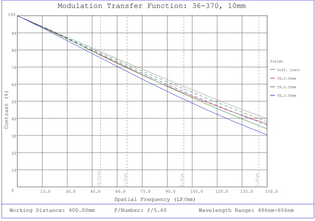
#36-370, 10mm FL f/5.6, Rugged Blue Series M12 Lens, Modulated Transfer Function (MTF) Plot, 400mm Working Distance, f5.6
