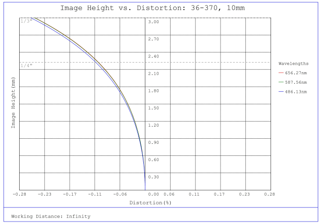
#36-370, 10mm FL f/5.6, Rugged Blue Series M12 Lens, Distortion Plot
