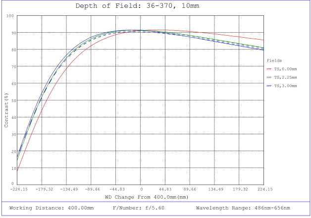
#36-370, 10mm FL f/5.6, Rugged Blue Series M12 Lens, Depth of Field Plot, 400mm Working Distance, f5.6
