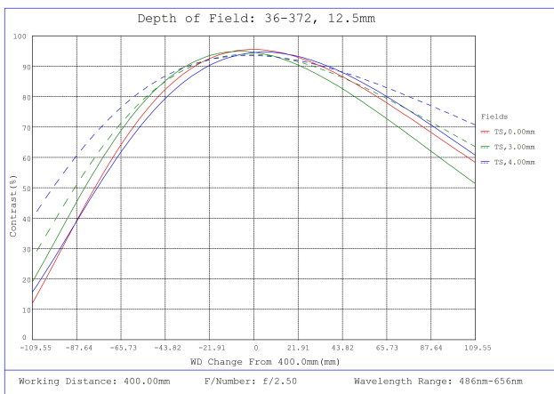
#36-372, 12.5mm FL f/2.5, Rugged Blue Series M12 Lens, Depth of Field Plot, 400mm Working Distance, f2.5
