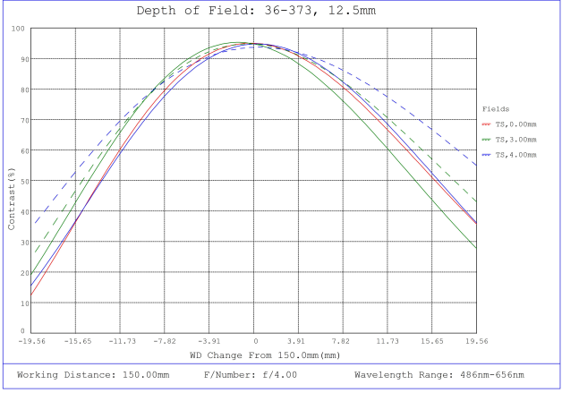
#36-373, 12.5mm FL f/4, Rugged Blue Series M12 Lens, Depth of Field Plot, 150mm Working Distance, f4
