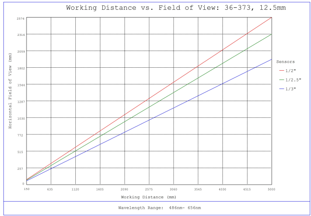
#36-373, 12.5mm FL f/4, Rugged Blue Series M12 Lens, Working Distance versus Field of View Plot
