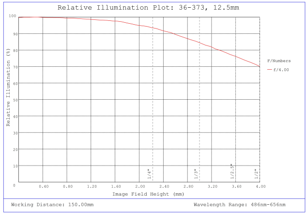
#36-373, 12.5mm FL f/4, Rugged Blue Series M12 Lens, Relative Illumination Plot
