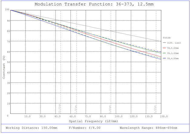
#36-373, 12.5mm FL f/4, Rugged Blue Series M12 Lens, Modulated Transfer Function (MTF) Plot, 150mm Working Distance, f4
