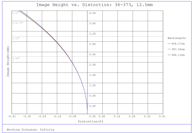
#36-373, 12.5mm FL f/4, Rugged Blue Series M12 Lens, Distortion Plot
