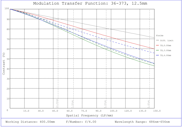
#36-373, 12.5mm FL f/4, Rugged Blue Series M12 Lens, Modulated Transfer Function (MTF) Plot, 400mm Working Distance, f4
