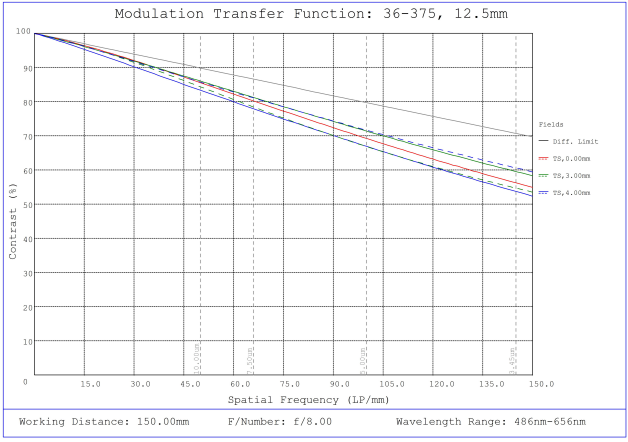
#36-375, 12.5mm FL f/8, Rugged Blue Series M12 Lens, Modulated Transfer Function (MTF) Plot, 150mm Working Distance, f8
