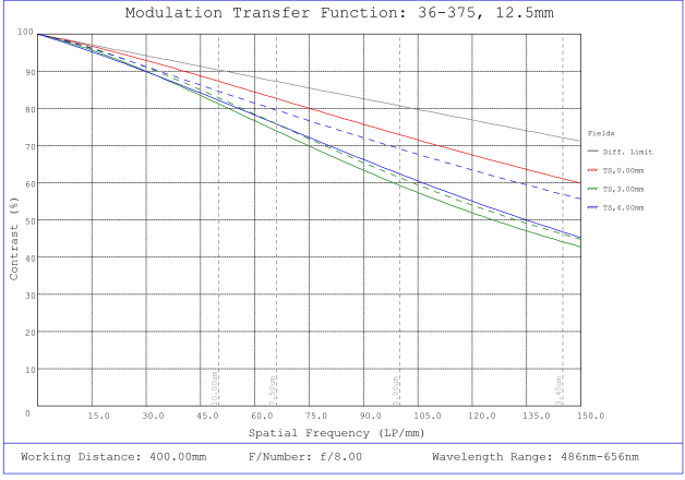
#36-375, 12.5mm FL f/8, Rugged Blue Series M12 Lens, Modulated Transfer Function (MTF) Plot, 400mm Working Distance, f8
