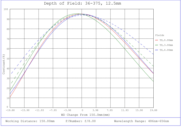
#36-375, 12.5mm FL f/8, Rugged Blue Series M12 Lens, Depth of Field Plot, 150mm Working Distance, f8
