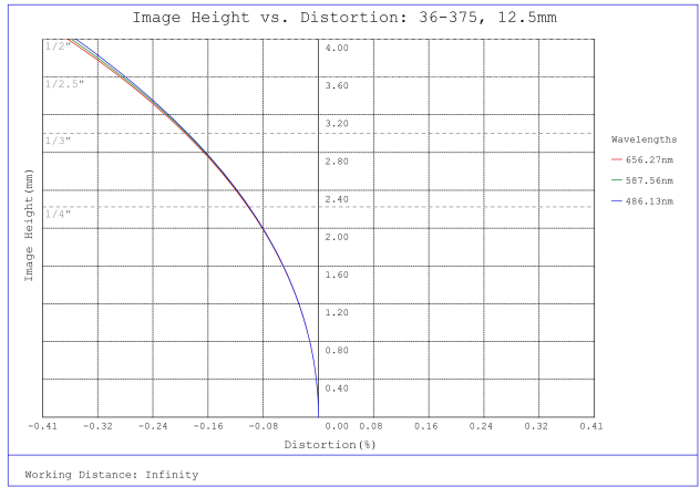
#36-375, 12.5mm FL f/8, Rugged Blue Series M12 Lens, Distortion Plot
