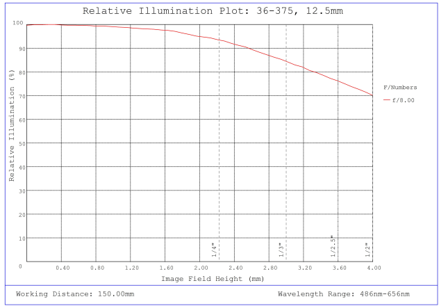
#36-375, 12.5mm FL f/8, Rugged Blue Series M12 Lens, Relative Illumination Plot
