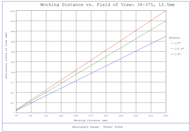
#36-375, 12.5mm FL f/8, Rugged Blue Series M12 Lens, Working Distance versus Field of View Plot
