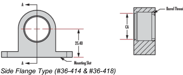
Side Flange Type (#36-414 & #36-418)
