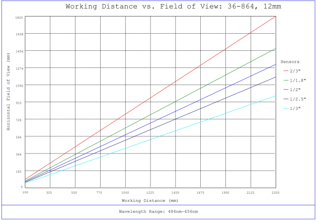
#36-864, 12mm f/11, 1000mm-∞ Primary WD, HRr Series Fixed Focal Length Lens, Working Distance versus Field of View Plot
