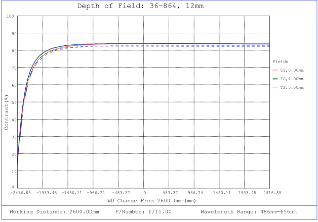
#36-864, 12mm f/11, 1000mm-∞ Primary WD, HRr Series Fixed Focal Length Lens, Depth of Field Plot, 2600mm Working Distance, f11
