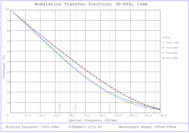
#36-864, 12mm f/11, 1000mm-∞ Primary WD, HRr Series Fixed Focal Length Lens, Modulated Transfer Function (MTF) Plot, 1000mm Working Distance, f11
