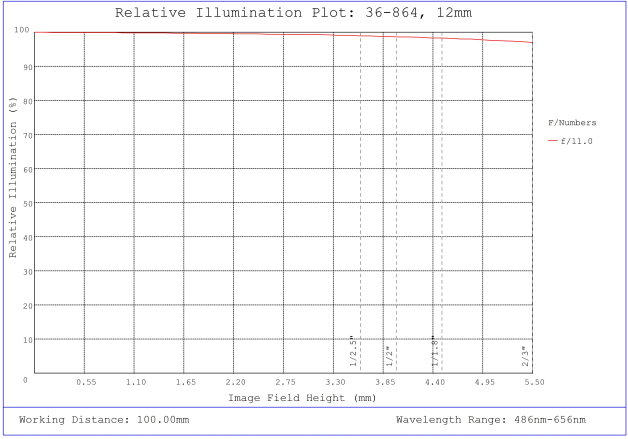
#36-864, 12mm f/11, 1000mm-∞ Primary WD, HRr Series Fixed Focal Length Lens, Relative Illumination Plot
