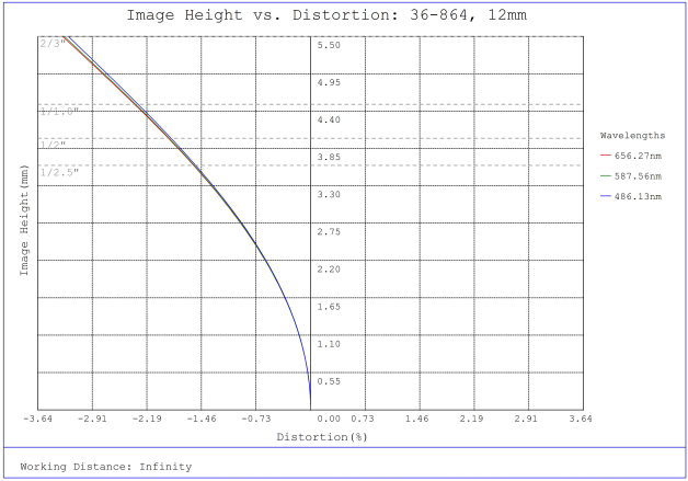
#36-864, 12mm f/11, 1000mm-∞ Primary WD, HRr Series Fixed Focal Length Lens, Distortion Plot
