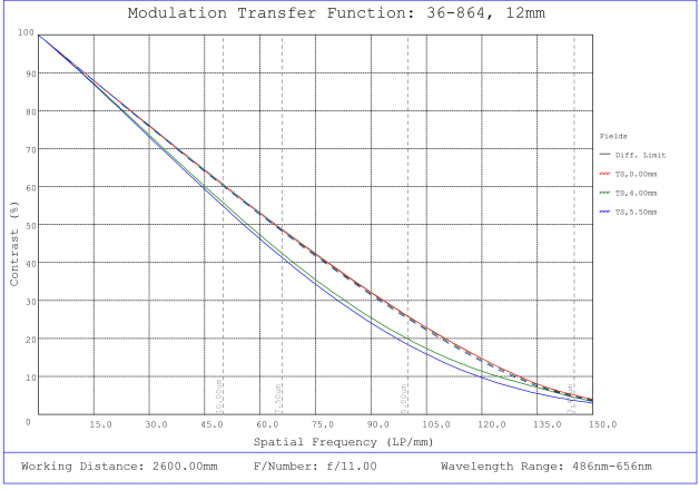
#36-864, 12mm f/11, 1000mm-∞ Primary WD, HRr Series Fixed Focal Length Lens, Modulated Transfer Function (MTF) Plot, 2600mm Working Distance, f11
