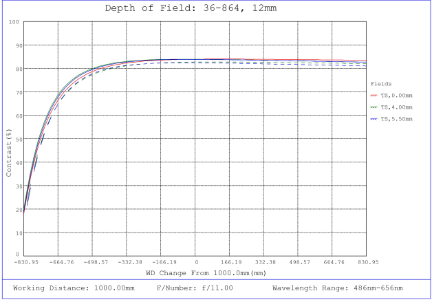
#36-864, 12mm f/11, 1000mm-∞ Primary WD, HRr Series Fixed Focal Length Lens, Depth of Field Plot, 1000mm Working Distance, f11
