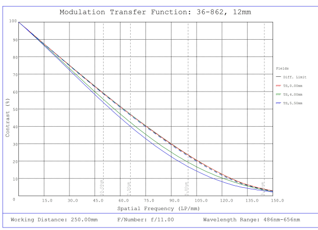
#36-862, 12mm f/11, 150-500mm Primary WD, HRr Series Fixed Focal Length Lens, Modulated Transfer Function (MTF) Plot, 250mm Working Distance, f11
