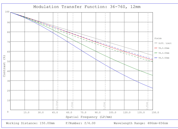
#36-760, 12mm f/4, 150-500mm Primary WD, HRI Series Fixed Focal Length Lens, Modulated Transfer Function (MTF) Plot, 150mm Working Distance, f4
