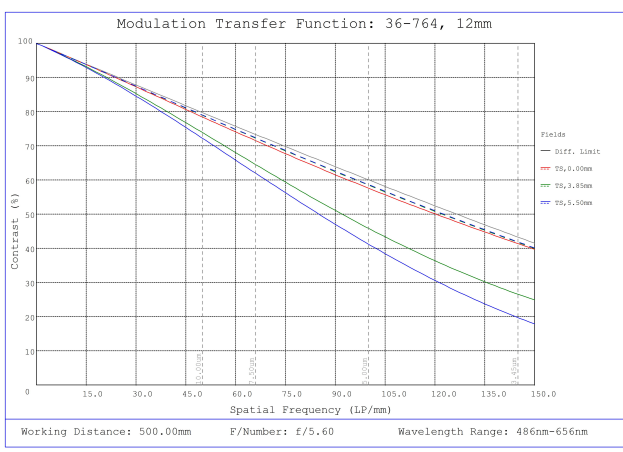
#36-764, 12mm f/5.6, 400-2000mm Primary WD, HRI Series Fixed Focal Length Lens, Modulated Transfer Function (MTF) Plot, 500mm Working Distance, f5.6
