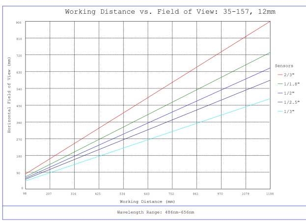
#35-157, 12mm, f/4 Cr Series Fixed Focal Length Lens, Working Distance versus Field of View Plot
