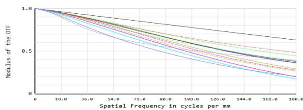
#22-835 - 12mm Focal Length, UAV Series Fixed Focal Length Lens, Modulated Transfer Function (MTF) Plot, Infinity Working Distance, f2.8
