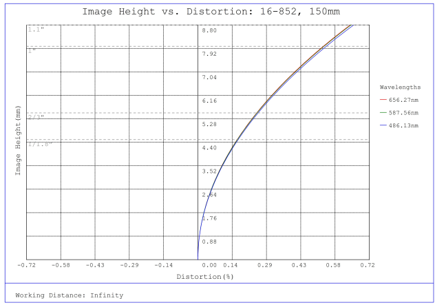
#16-852, 150mm, f/4 Athermal Lens, Distortion Plot
