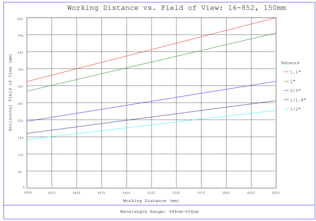
#16-852, 150mm, f/4 Athermal Lens, Working Distance versus Field of View Plot
