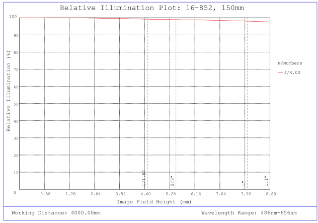
#16-852, 150mm, f/4 Athermal Lens, Relative Illumination Plot
