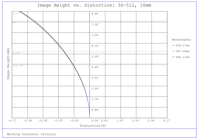
#36-512, 16mm f/2.8, HPr Series Fixed Focal Length Lens, Distortion Plot
