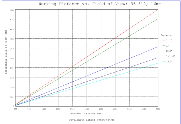
#36-512, 16mm f/2.8, HPr Series Fixed Focal Length Lens, Working Distance versus Field of View Plot
