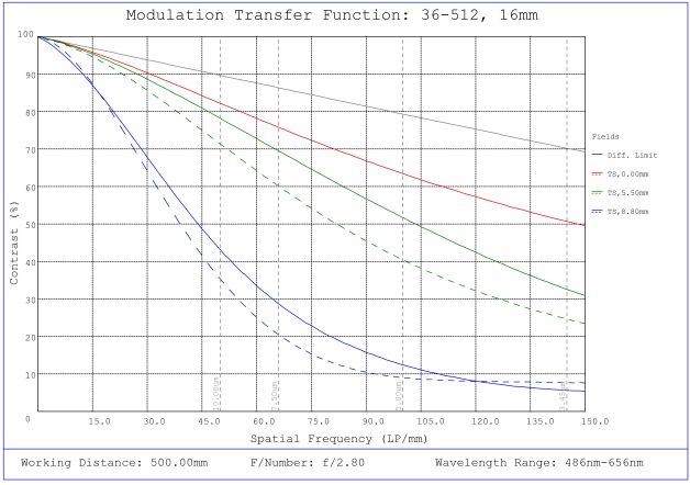
#36-512, 16mm f/2.8, HPr Series Fixed Focal Length Lens, Modulated Transfer Function (MTF) Plot, 500mm Working Distance, f2.8
