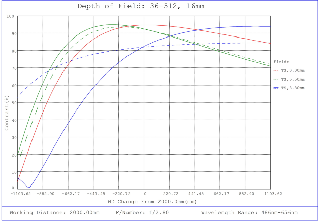
#36-512, 16mm f/2.8, HPr Series Fixed Focal Length Lens, Depth of Field Plot, 2000mm Working Distance, f2.8
