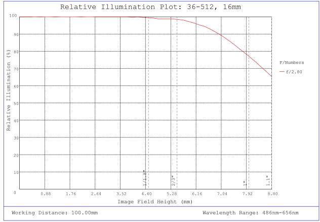
#36-512, 16mm f/2.8, HPr Series Fixed Focal Length Lens, Relative Illumination Plot
