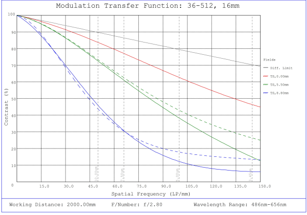
#36-512, 16mm f/2.8, HPr Series Fixed Focal Length Lens, Modulated Transfer Function (MTF) Plot, 2000mm Working Distance, f2.8
