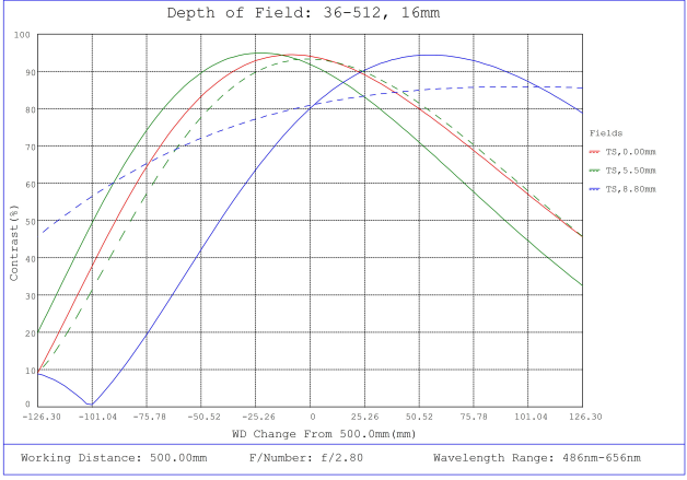
#36-512, 16mm f/2.8, HPr Series Fixed Focal Length Lens, Depth of Field Plot, 500mm Working Distance, f2.8
