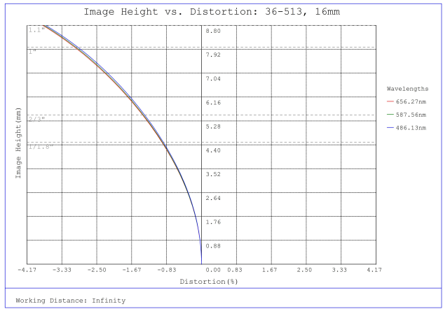
#36-513, 16mm f/4, HPr Series Fixed Focal Length Lens, Distortion Plot
