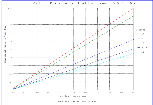
#36-513, 16mm f/4, HPr Series Fixed Focal Length Lens, Working Distance versus Field of View Plot
