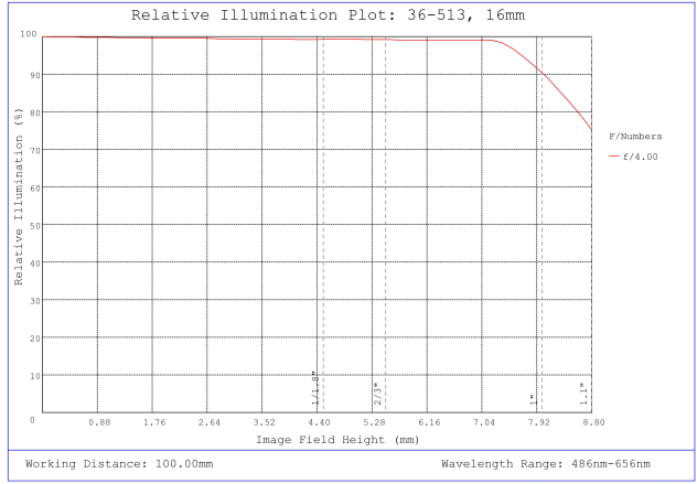
#36-513, 16mm f/4, HPr Series Fixed Focal Length Lens, Relative Illumination Plot
