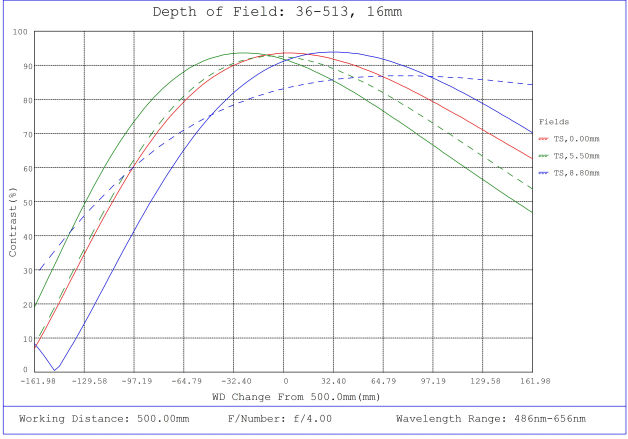
#36-513, 16mm f/4, HPr Series Fixed Focal Length Lens, Depth of Field Plot, 500mm Working Distance, f4
