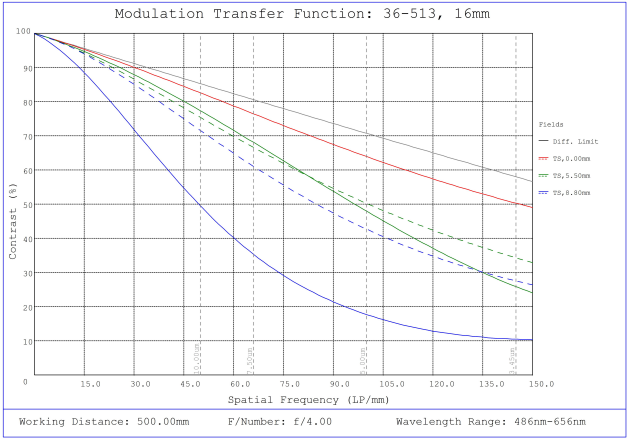
#36-513, 16mm f/4, HPr Series Fixed Focal Length Lens, Modulated Transfer Function (MTF) Plot, 500mm Working Distance, f4
