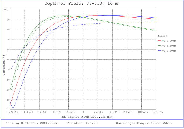
#36-513, 16mm f/4, HPr Series Fixed Focal Length Lens, Depth of Field Plot, 2000mm Working Distance, f4
