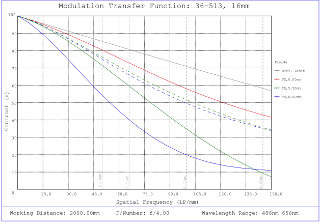
#36-513, 16mm f/4, HPr Series Fixed Focal Length Lens, Modulated Transfer Function (MTF) Plot, 2000mm Working Distance, f4
