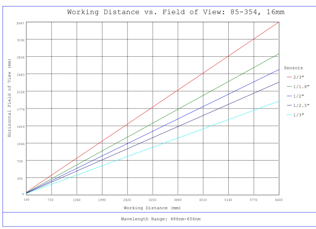
#85-354, 16mm, f/11 Ci Series Fixed Focal Length Lens, Working Distance versus Field of View Plot
