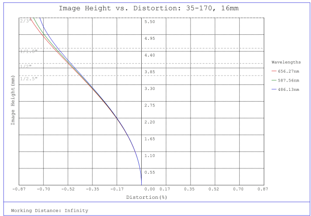
#35-170, 16mm, f/16 Cr Series Fixed Focal Length Lens, Distortion Plot
