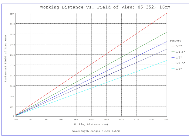
#85-352, 16mm, f/5.6 Ci Series Fixed Focal Length Lens, Working Distance versus Field of View Plot
