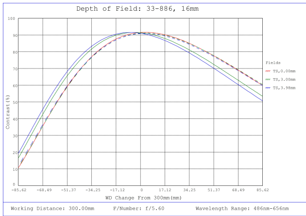
#33-886, 16mm, f/5.6 UCi Series Fixed Focal Length Lens, Depth of Field Plot, 300mm Working Distance, f5.6
