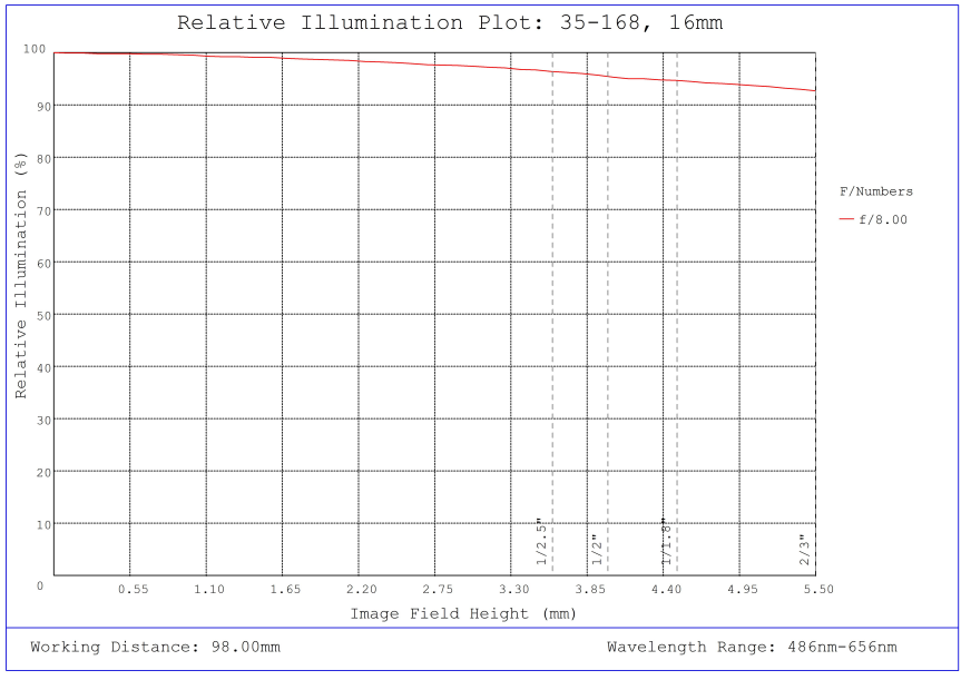
#35-168, 16mm, f/8 Cr Series Fixed Focal Length Lens, Relative Illumination Plot
