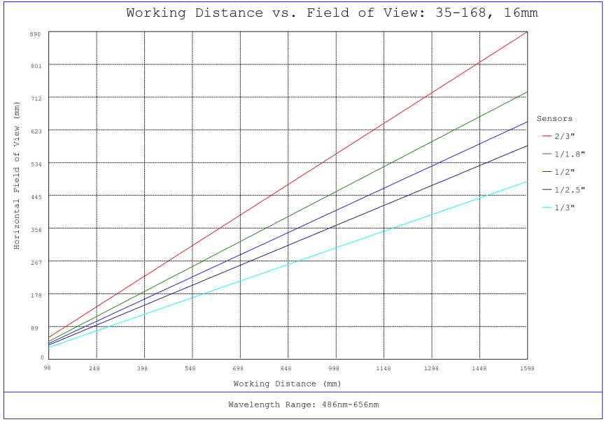
#35-168, 16mm, f/8 Cr Series Fixed Focal Length Lens, Working Distance versus Field of View Plot
