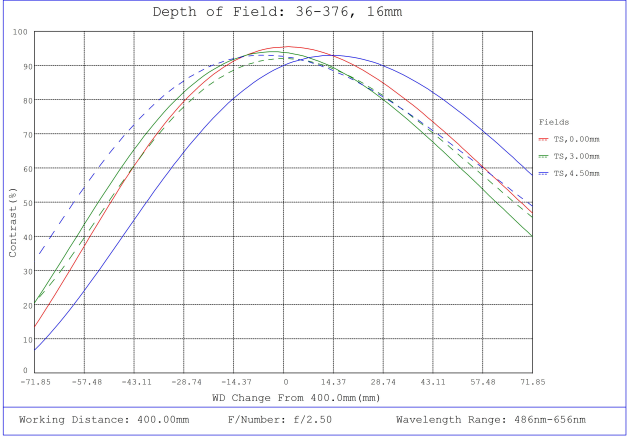
#36-376, 16mm FL f/2.5 Rugged Blue Series M12 Lens, Depth of Field Plot, 400mm Working Distance, f2.5
