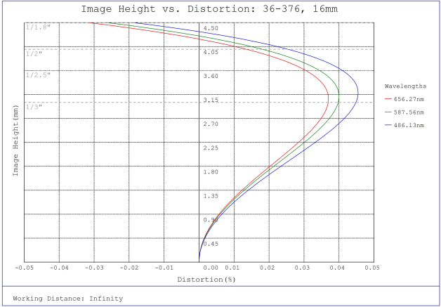
#36-376, 16mm FL f/2.5 Rugged Blue Series M12 Lens, Distortion Plot
