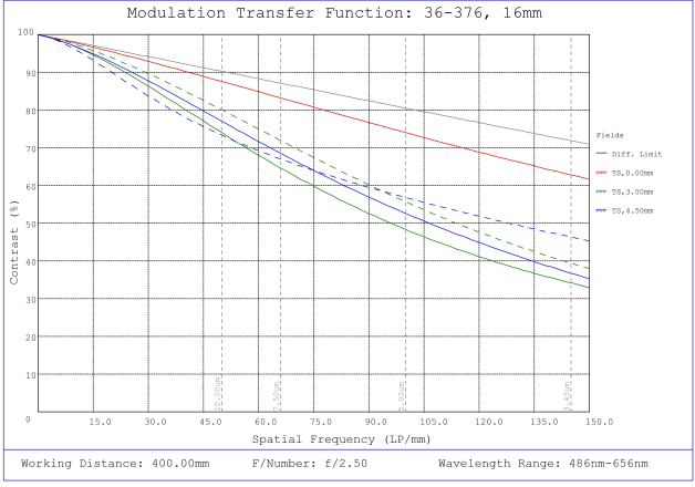
#36-376, 16mm FL f/2.5 Rugged Blue Series M12 Lens, Modulated Transfer Function (MTF) Plot, 400mm Working Distance, f2.5
