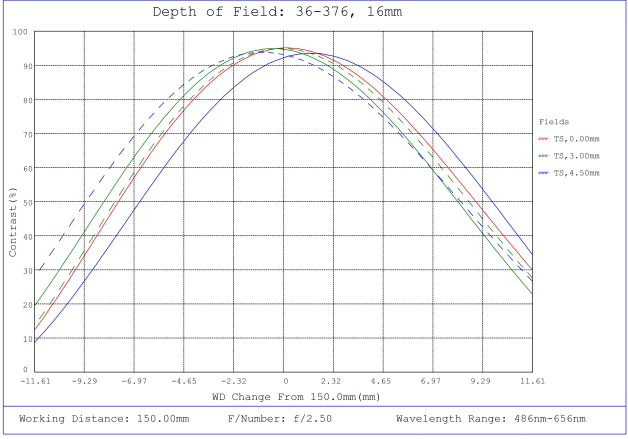
#36-376, 16mm FL f/2.5 Rugged Blue Series M12 Lens, Depth of Field Plot, 150mm Working Distance, f2.5
