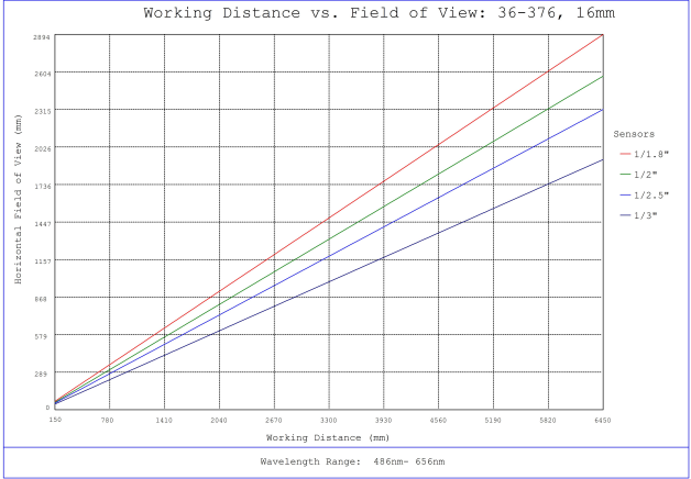
#36-376, 16mm FL f/2.5 Rugged Blue Series M12 Lens, Working Distance versus Field of View Plot
