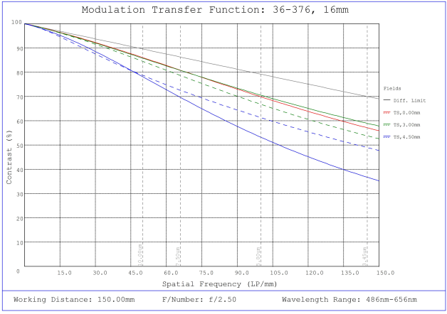
#36-376, 16mm FL f/2.5 Rugged Blue Series M12 Lens, Modulated Transfer Function (MTF) Plot, 150mm Working Distance, f2.5
