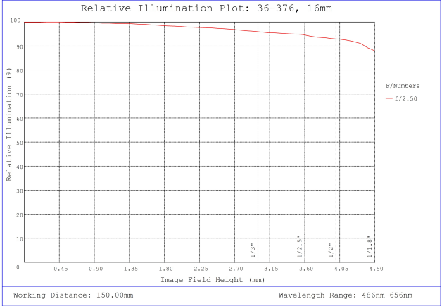
#36-376, 16mm FL f/2.5 Rugged Blue Series M12 Lens, Relative Illumination Plot
