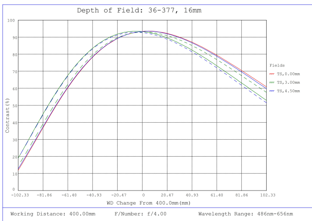
#36-377, 16mm FL f/4.0 Rugged Blue Series M12 Lens, Depth of Field Plot, 400mm Working Distance, f4
