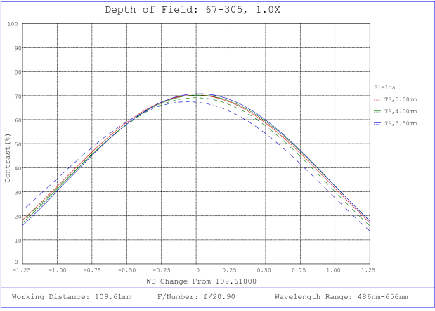
#67-305, 1X, 110mm WD, In-Line CompactTL™ Telecentric Lens, Depth of Field Plot, 110mm Working Distance, f20.9
