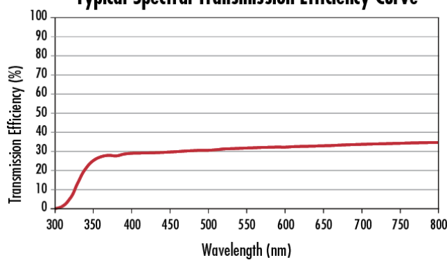
Typical Spectral Transmission Efficiency Curve
