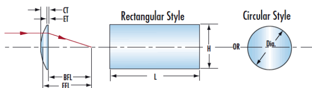
Circular And Rectangular Cylinder Lenses
