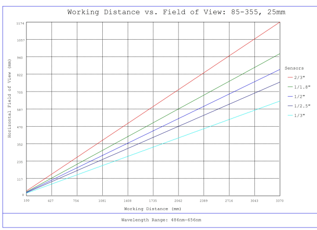
#85-355, 25mm, f/1.4 Ci Series Fixed Focal Length Lens, Working Distance versus Field of View Plot
