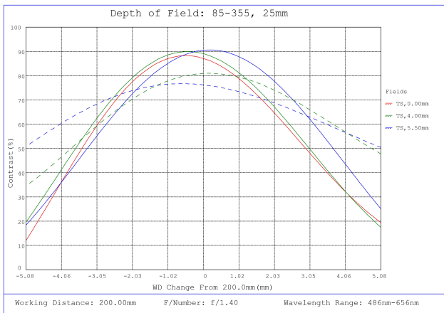
#85-355, 25mm, f/1.4 Ci Series Fixed Focal Length Lens, Depth of Field Plot, 200mm Working Distance, f1.4
