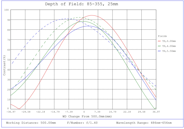
#85-355, 25mm, f/1.4 Ci Series Fixed Focal Length Lens, Depth of Field Plot, 500mm Working Distance, f1.4
