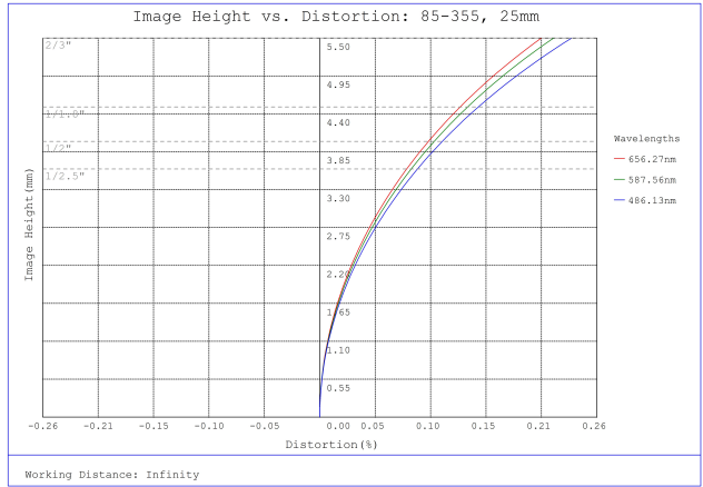
#85-355, 25mm, f/1.4 Ci Series Fixed Focal Length Lens, Distortion Plot
