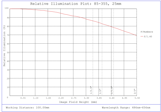
#85-355, 25mm, f/1.4 Ci Series Fixed Focal Length Lens, Relative Illumination Plot
