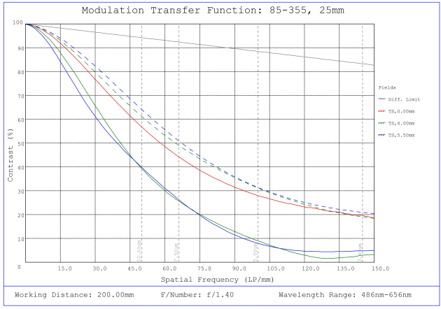
#85-355, 25mm, f/1.4 Ci Series Fixed Focal Length Lens, Modulated Transfer Function (MTF) Plot, 200mm Working Distance, f1.4
