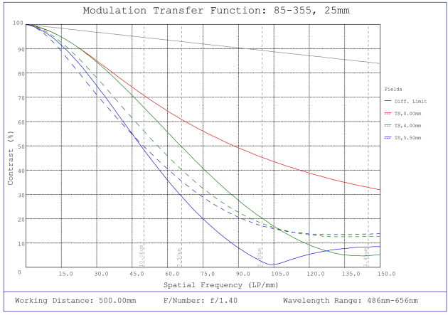
#85-355, 25mm, f/1.4 Ci Series Fixed Focal Length Lens, Modulated Transfer Function (MTF) Plot, 500mm Working Distance, f1.4
