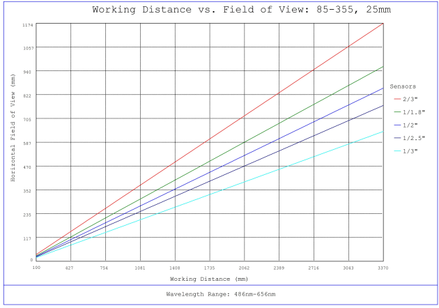
#85-355, 25mm, f/1.4 Ci Series Fixed Focal Length Lens, Working Distance versus Field of View Plot
